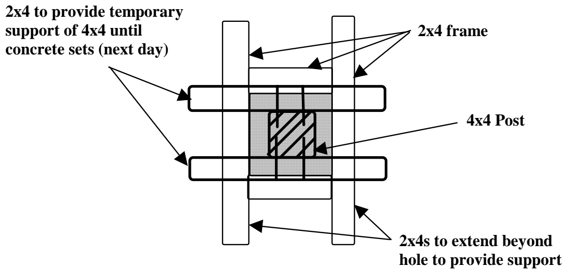
Figure 8 Concrete Foundation/Pier Construction (Where Required)
