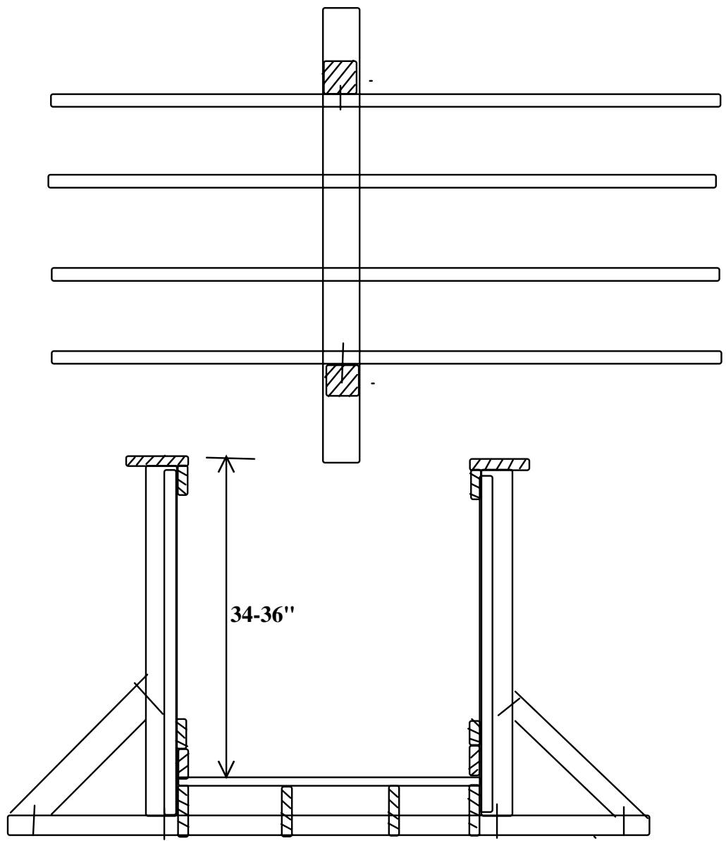
Figure 10 Ramp Gound Termination
